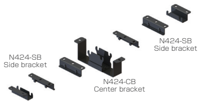
N424 K2 Double opening cable management metal fitting
