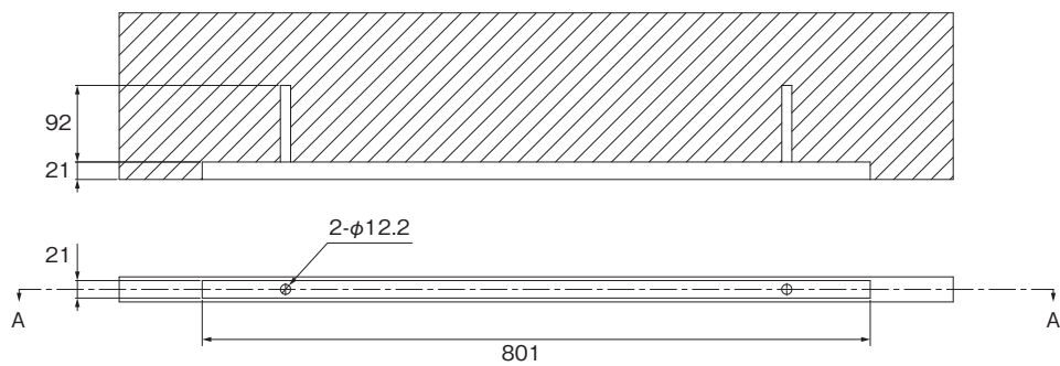
Reference diagram for shelf digging dimensions
