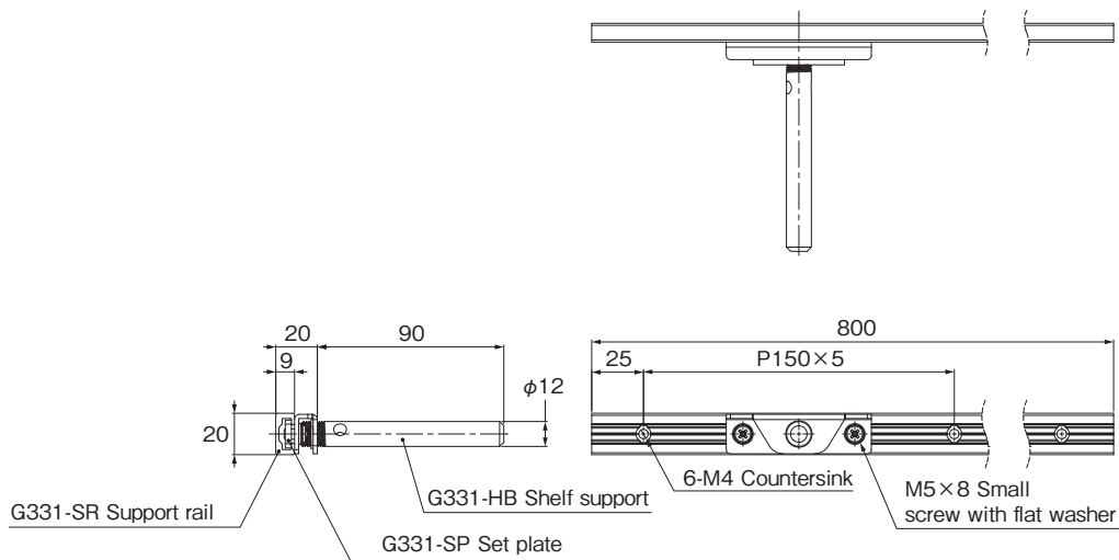
Reference diagram for shelf digging dimensions
